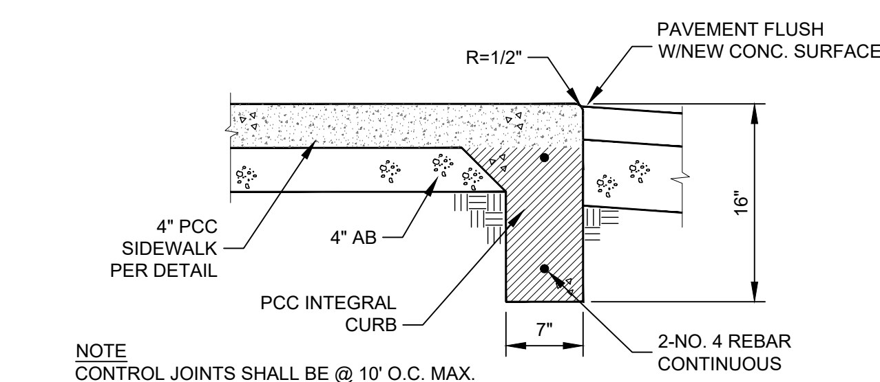
6 TYPE A2: INTEGRAL SIDEWALK & CURB NTS
