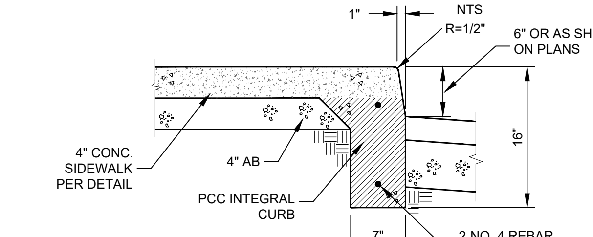
4 PCC SIDEWALK DETAIL NTS
