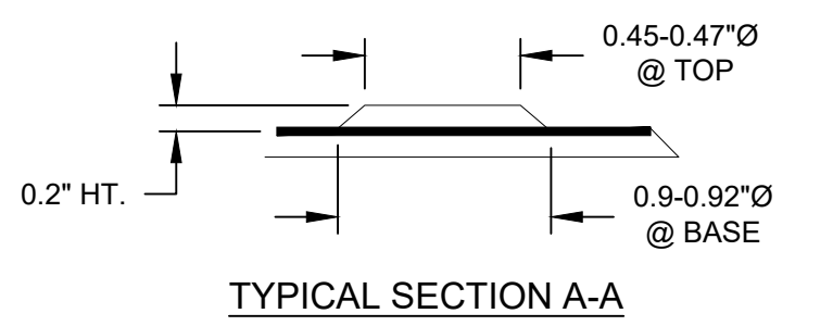
10 TRUNCATED DOMES NTS
