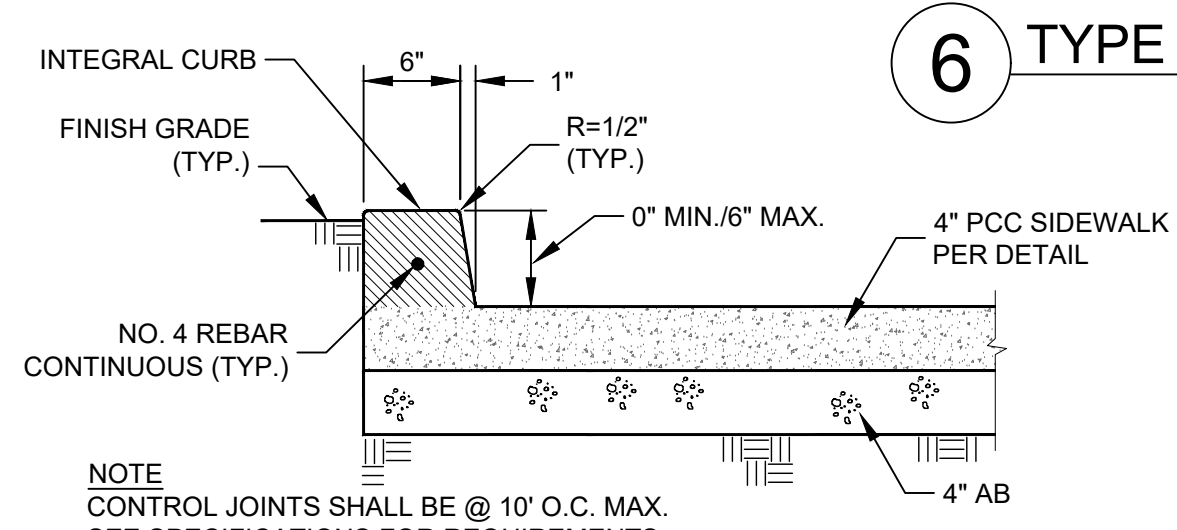
12 TYPE A3: INTEGRAL CURB @ LANDSCAPE NTS
