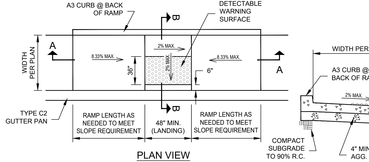
8 TYPE C2: INTEGRAL PCC GUTTER W/FLUSH CURB NTS
