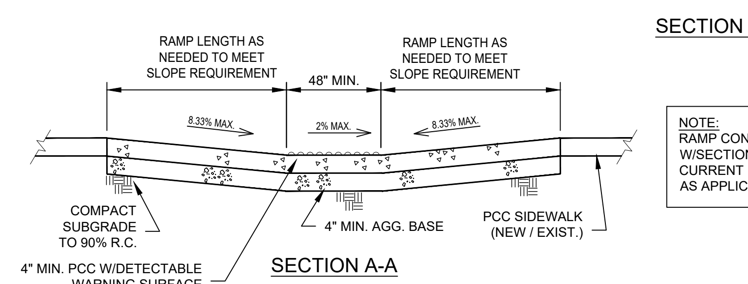
7 CURB RAMP TYPE C DETAIL NTS
