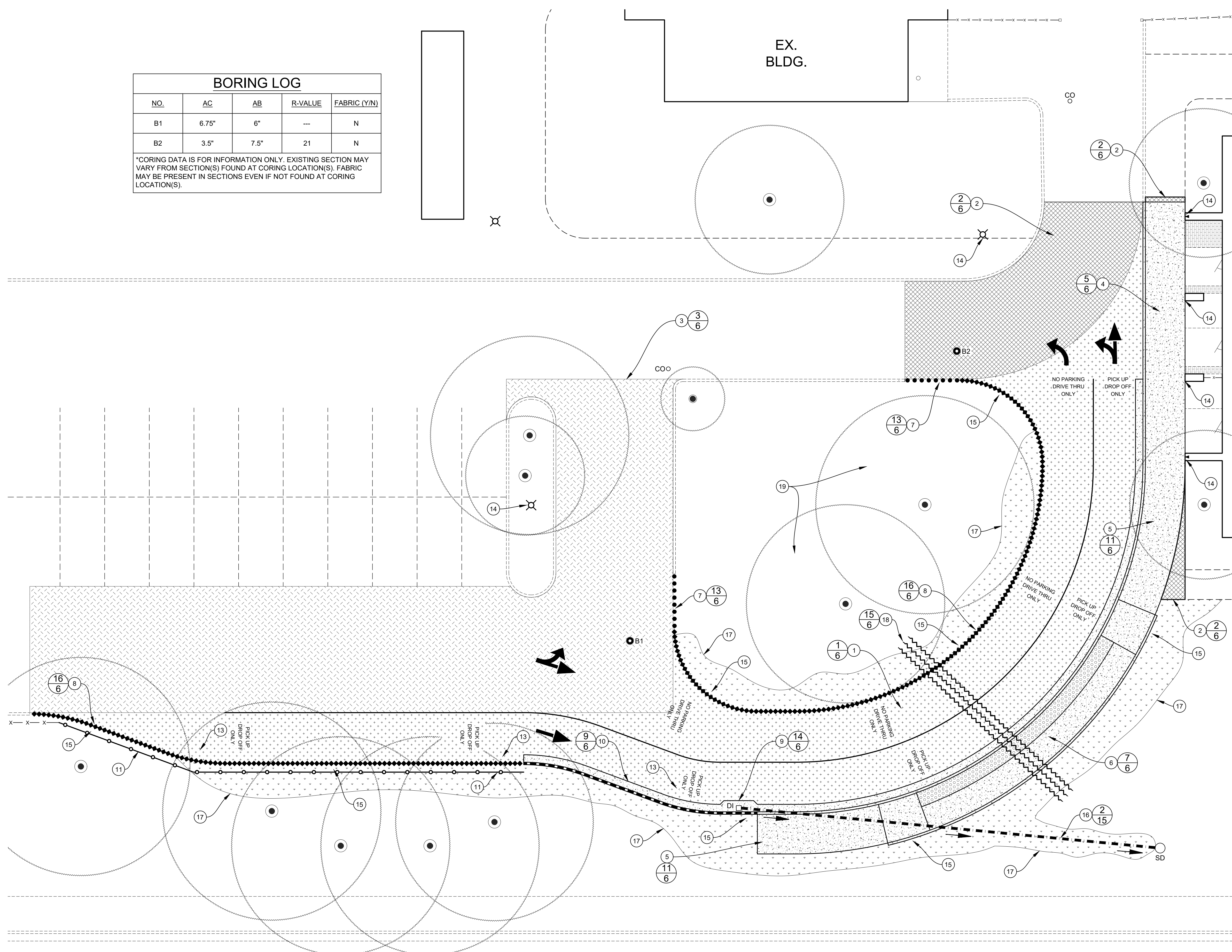
AREA OF ENLARGEMENT - SITE PLAN 1" = 10'
