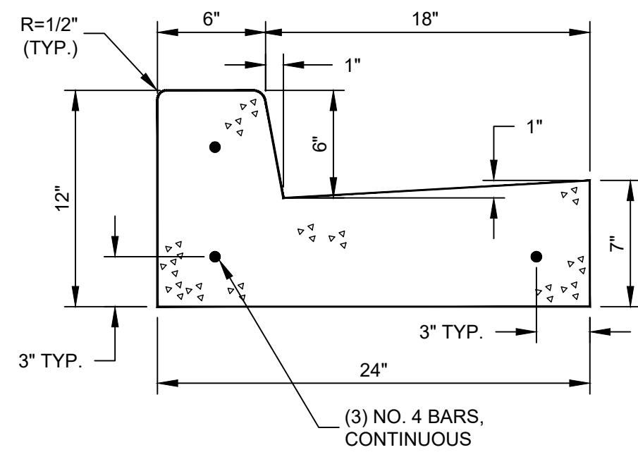
9 PCC CURB & GUTTER DETAIL
