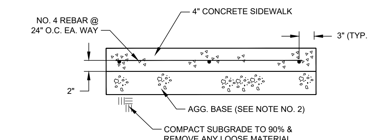
4 PCC SIDEWALK DETAIL NTS
