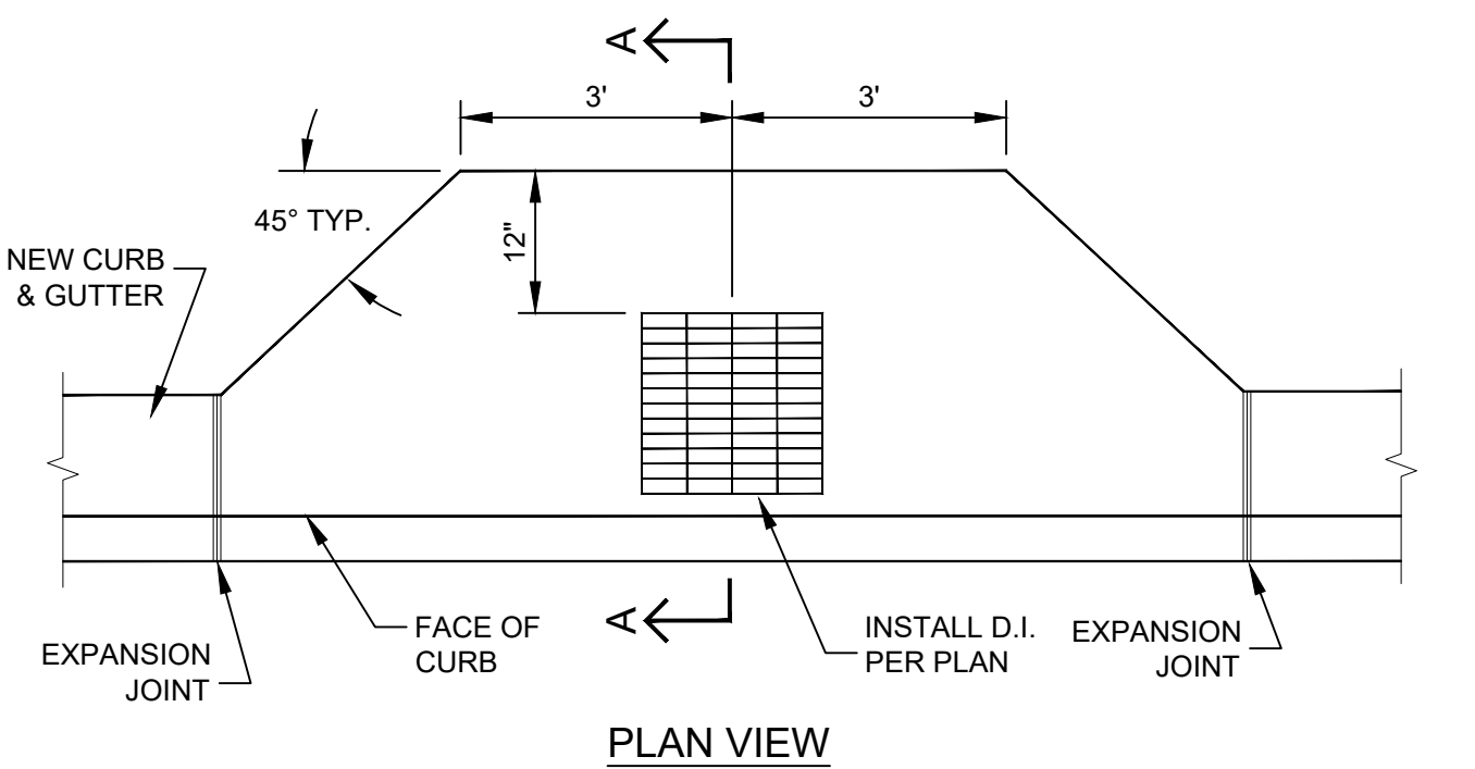
15 TYPICAL TRENCH BACKFILL DETAIL NTS
