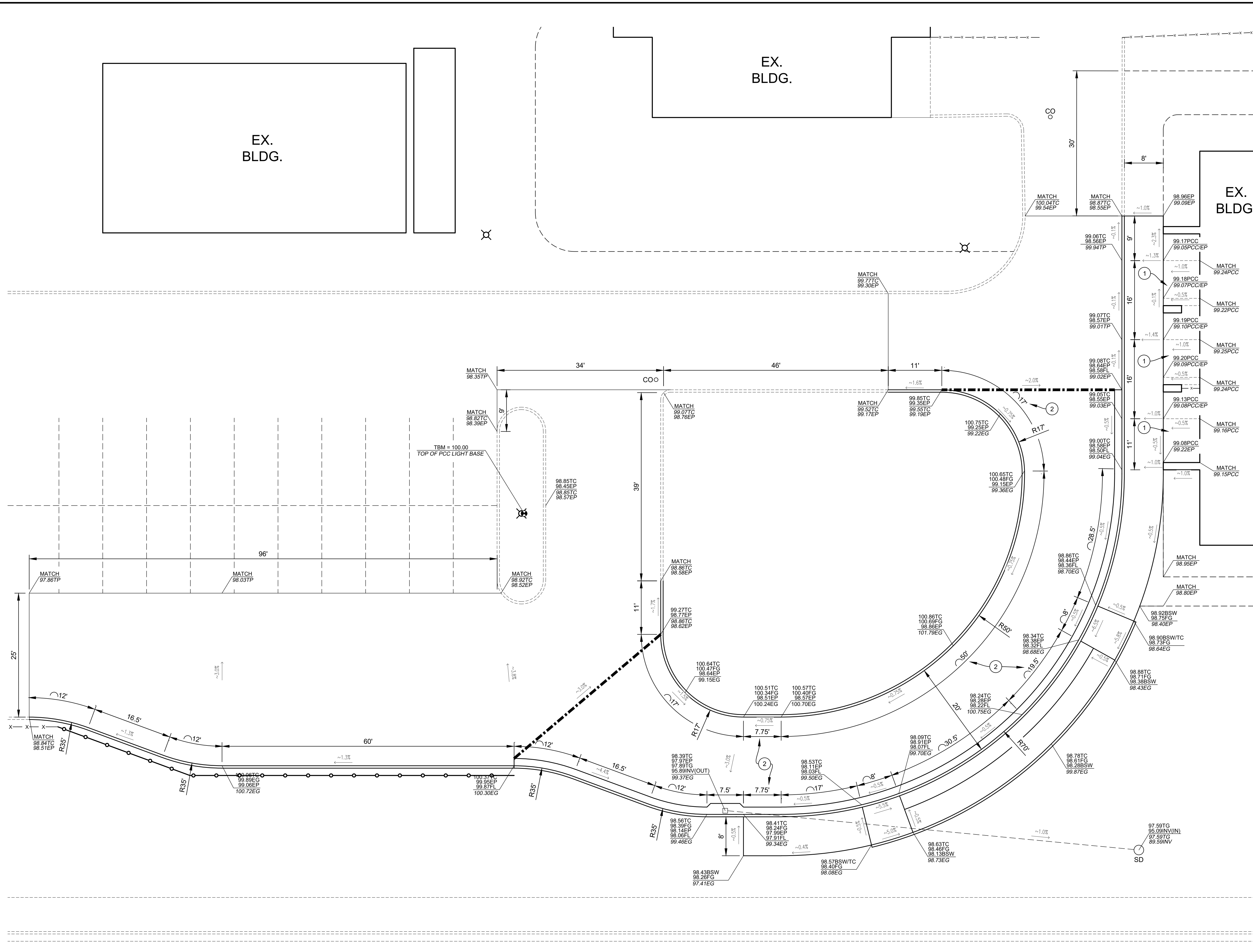
AREA OF ENLARGEMENT - GRADING PLAN 1" = 10'
