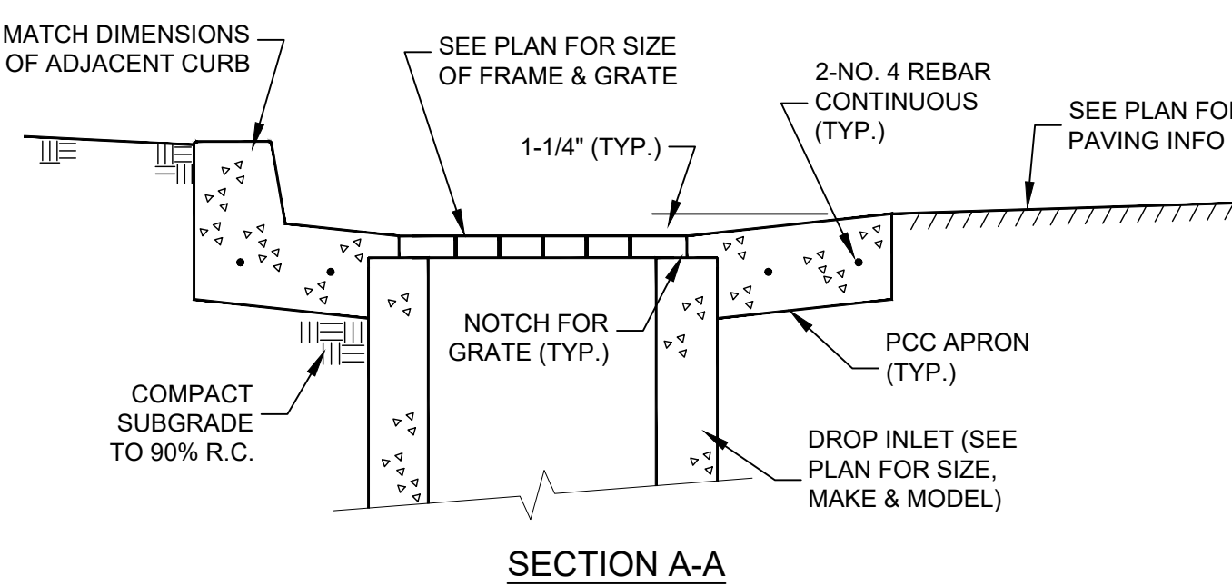
14 PCC APRON @ DROP INLET NTS
