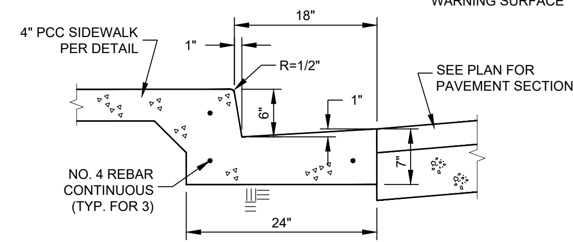
10 TRUNCATED DOMES NTS
