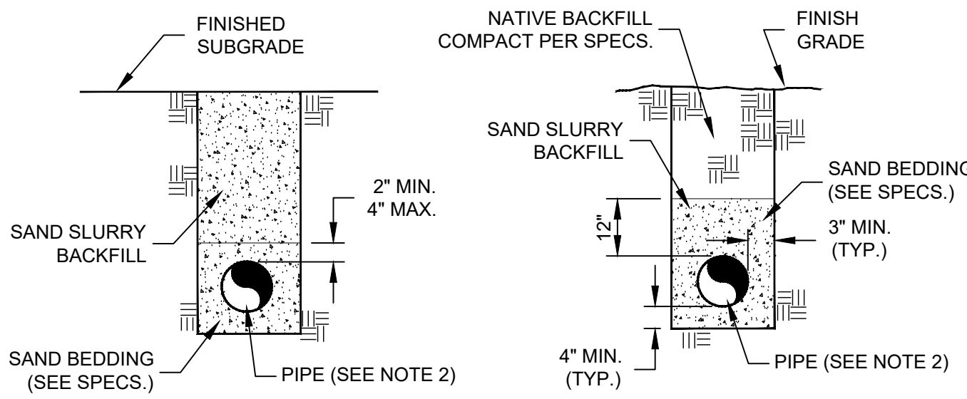
BACKFILL UNDER PAVEMENT BACKFILL UNDER LANDSCAPE
