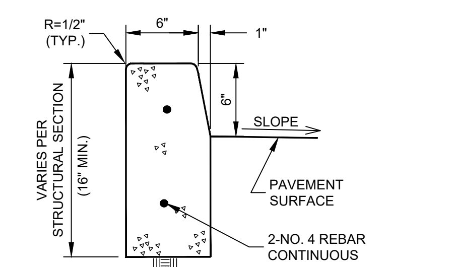
13 PCC CURB DETAIL NTS
