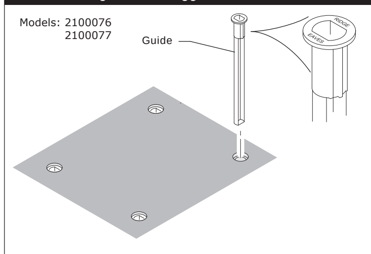
Figure B4 - Toggle Bolt Assembly
