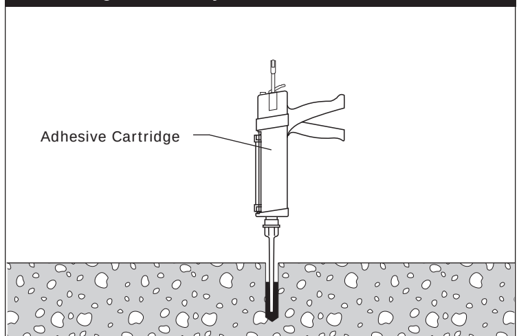
Figure C3 - Inject Adhesive into Holes
