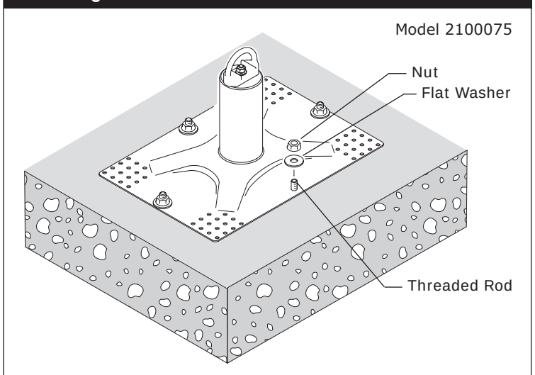
Figure C4 - Install Chemical Anchor Nuts
