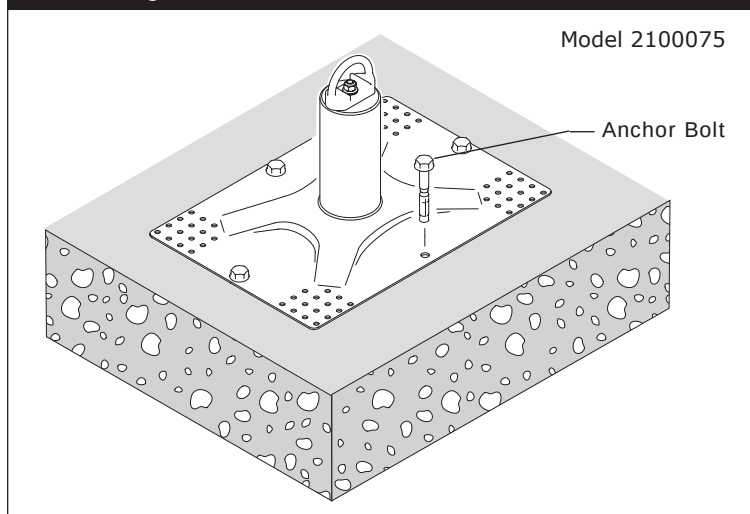
Figure C5 - Install Mechanical Anchors
