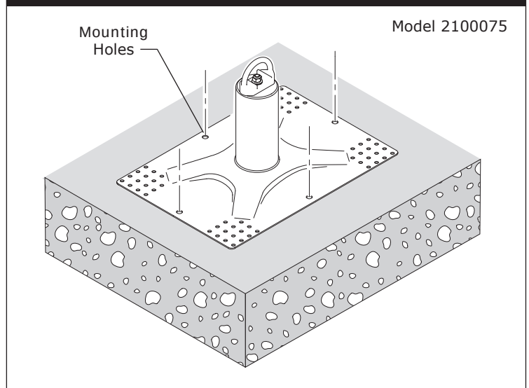
Figure C2 - Position Roof Anchor
