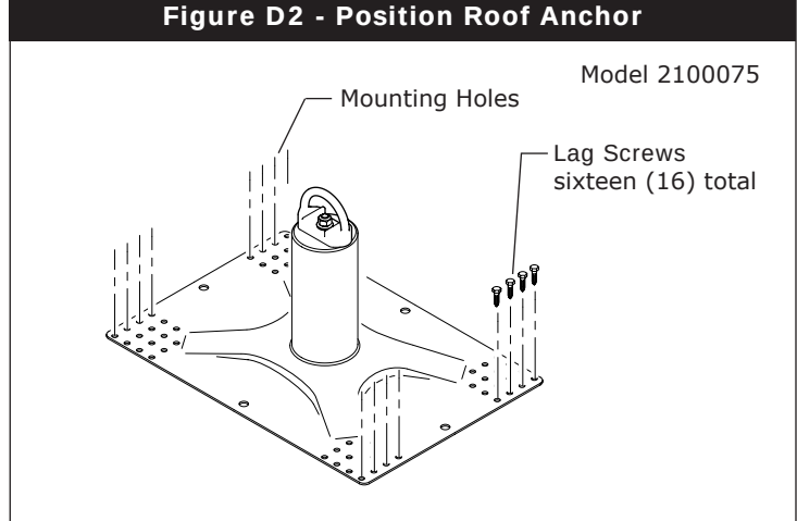
Figure D2 - Position Roof Anchor
