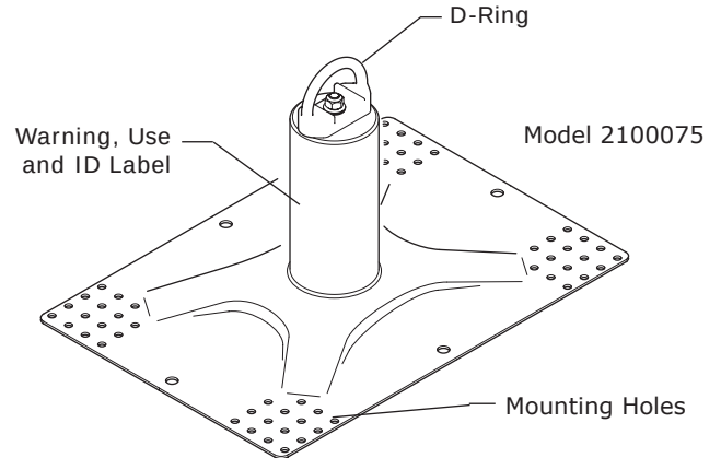
Figure D1 - Roof Anchor
