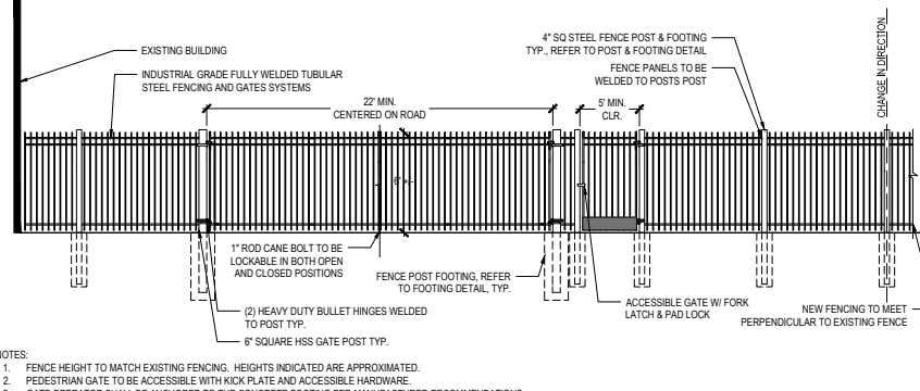
11 SOUTH GATE 2 ELEVATION NTS
