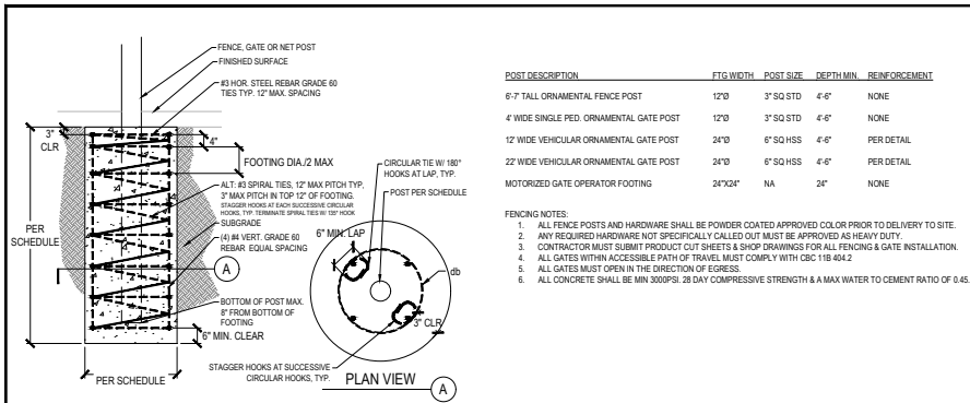
1 FENCE POST AND FOOTINGS NTS
