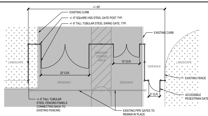
3 NORTH GATES 2 ENLARGMENT SCALE: 1/8" = 1'-0"
