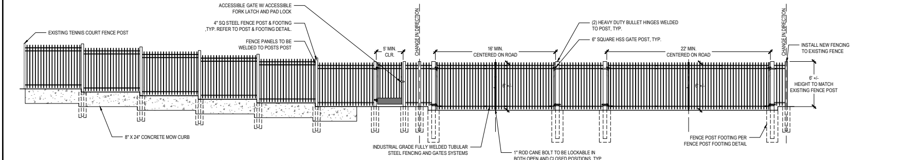
5 NORTH GATES 1 ELEVATION NTS
