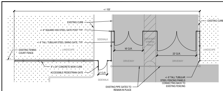
1 NORTH GATES 1 ENLARGMENT SCALE: 1/8" = 1'-0"
