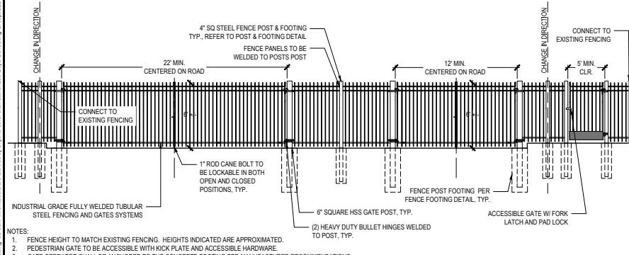
9 NORTH GATES 2 ELEVATION NTS
