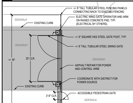
1 NORTH GATES 1 ENLARGMENT SCALE: 1/8" = 1'-0"
