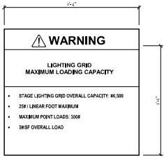
7 WARNING SIGNAGE AT LIGHTING GRID 1 1/2\"/>
