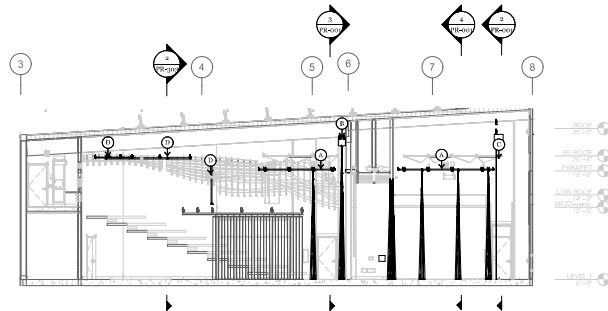
1 LOADING DIAGRAM - PRODUCTION RIGGING - CENTERLINE SECTION 1/8" = 1'-0"
