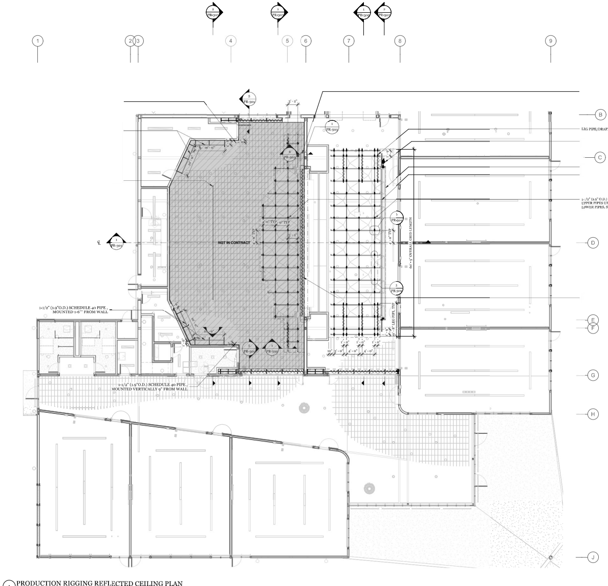
1 PRODUCTION RIGGING REFLECTED CEILING PLAN 1/8" = 1'-0"
