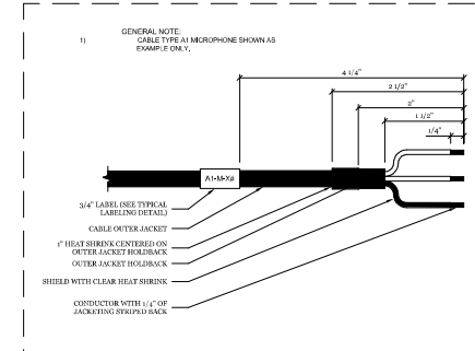
4 TYPICAL WIRE TERMINATION PREP
