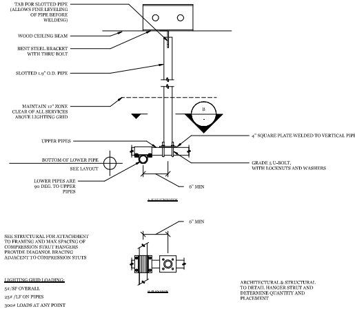
2 TYPICAL COMPRESSION STRUT LIGHTING GRID HANGER 1 1/2\"/>
