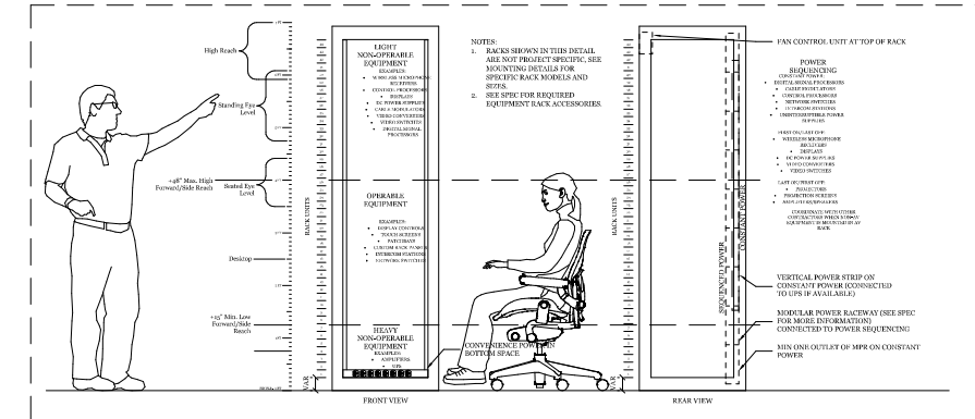
1 RACK ELEVATION GUIDELINES
