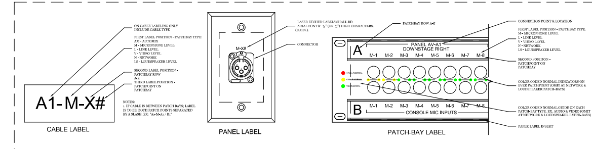
2 TYPICAL LABELING DETAIL
