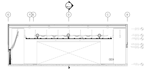
4 LOADING DIAGRAM - PRODUCTION RIGGING - LIGHTING GRID ELEVATION 1/8" = 1'-0"
