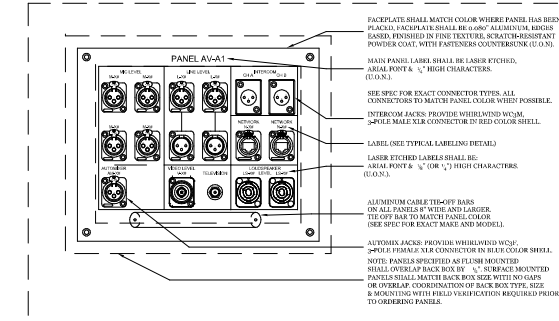
3 TYPICAL MULTIO PANEL
