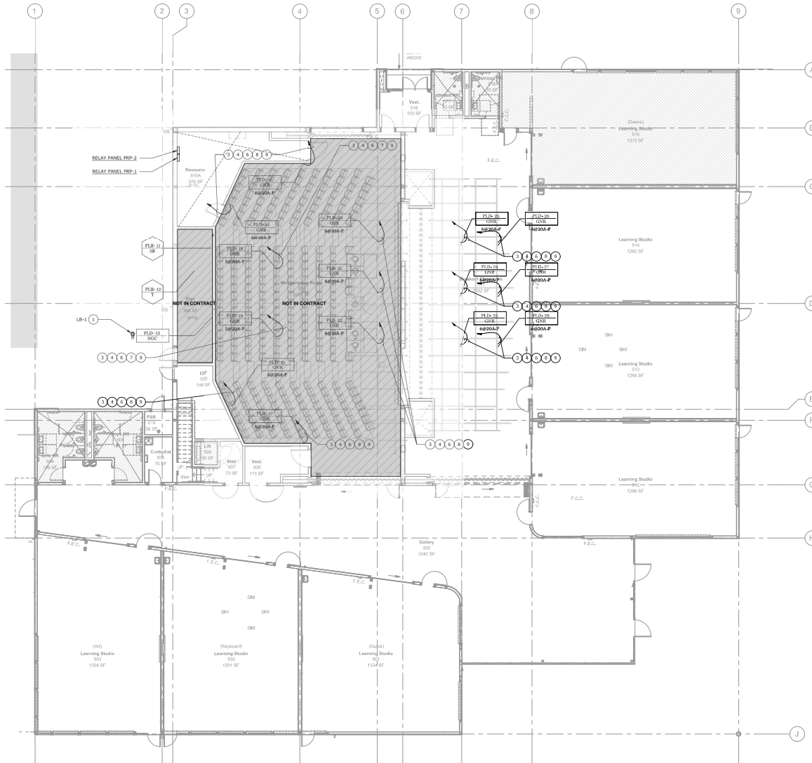
PRODUCTION LIGHTING PLAN AT MEZZANINE LEVEL - ELECTRICAL SCALE: 1/8" = 1'-0"
