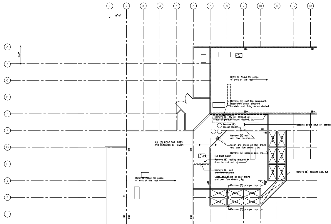
① Enlarged Roof Plan: Demo 1/16" = 1'-0"
