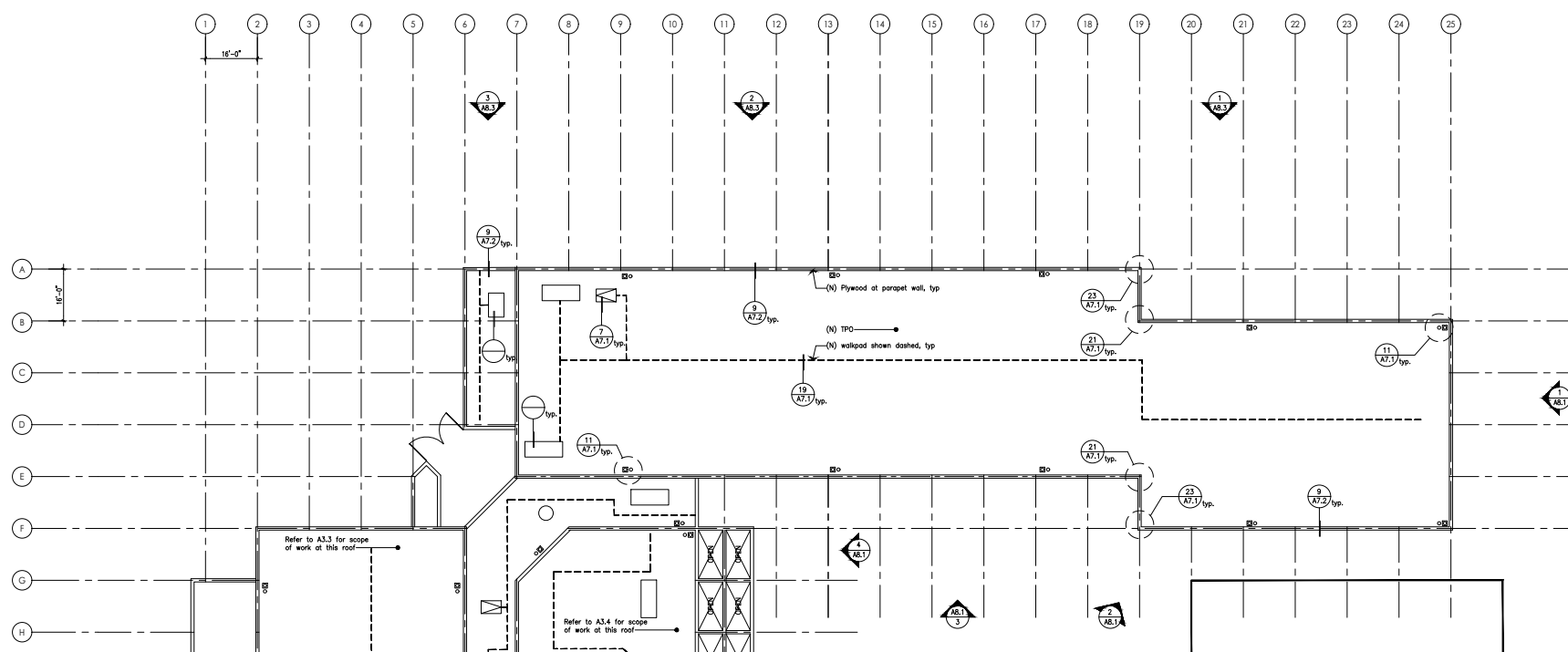
1 Roof Plan: Proposed
