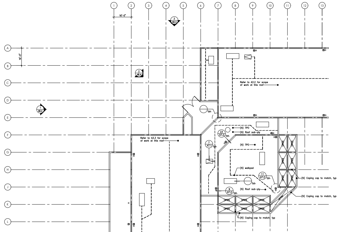
① Enlarged Roof Plan: Proposed 1/16" = 1'-0"
